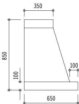
Hotte murale configuration standard
